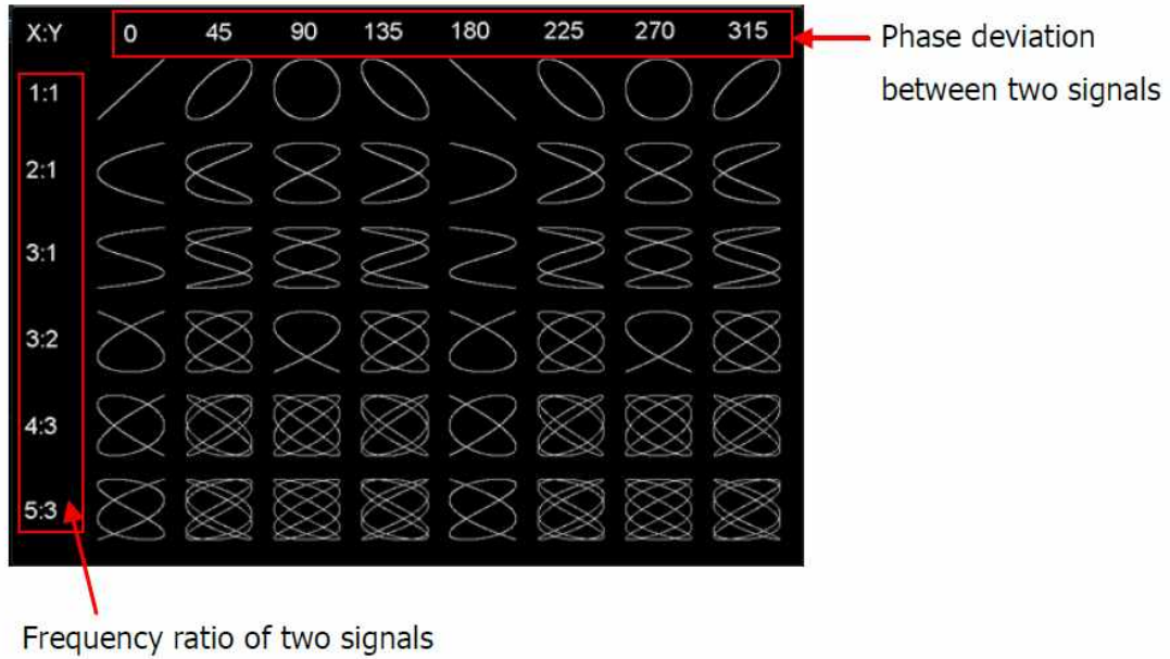
Figure 6-7 Lissajous Schematic Diagrams
